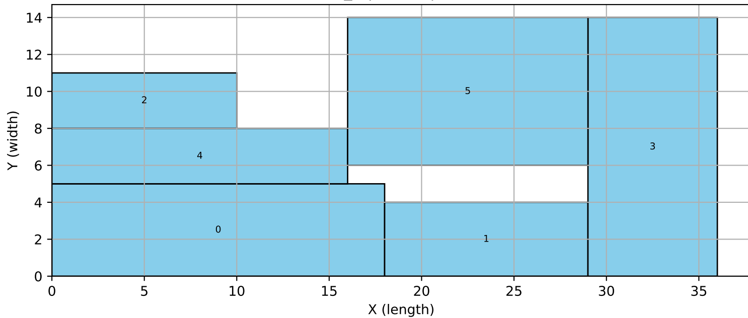
6_7 | reagg | MIP
