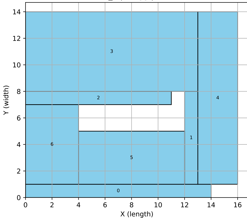
7_4 | reagg | MIP
