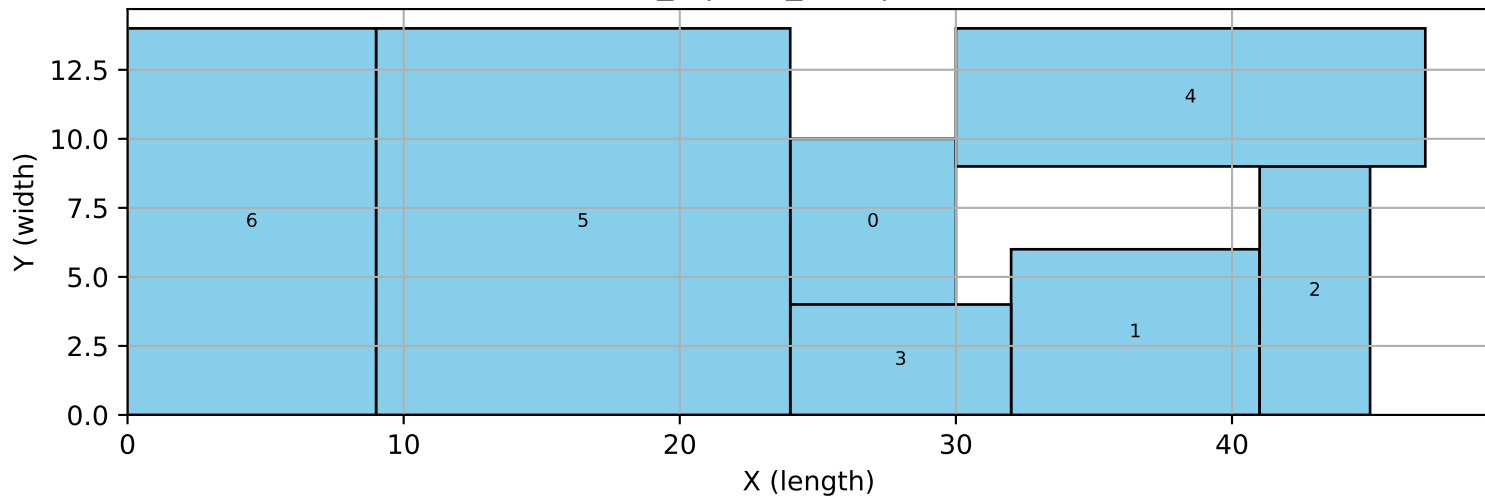
7_9 | tres_sym | bigm
