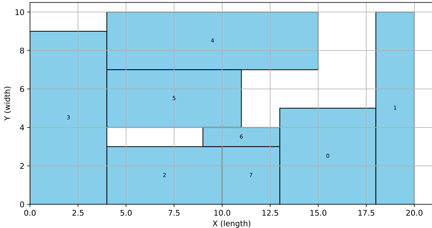
8_2 | tres_sym | bigm
