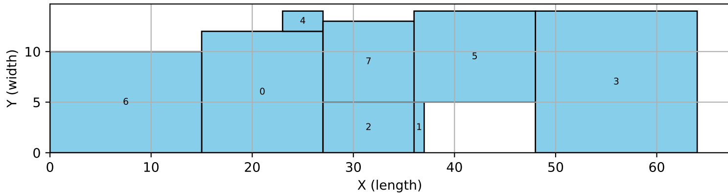
8_4 | reagg_tres | MIP
