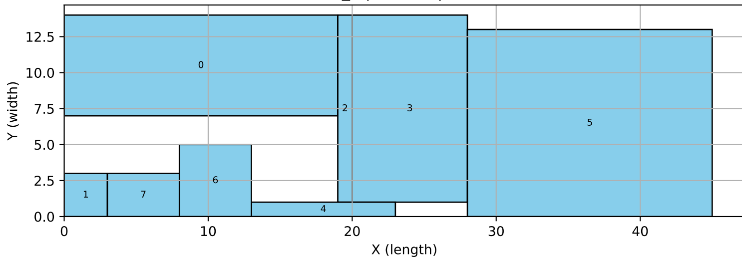
8_6 | altered | hull
