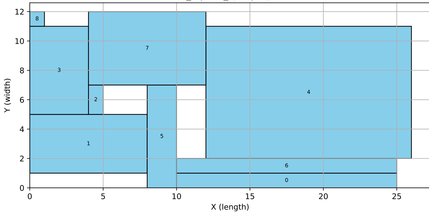
9_1 | tres_sym | bigm
