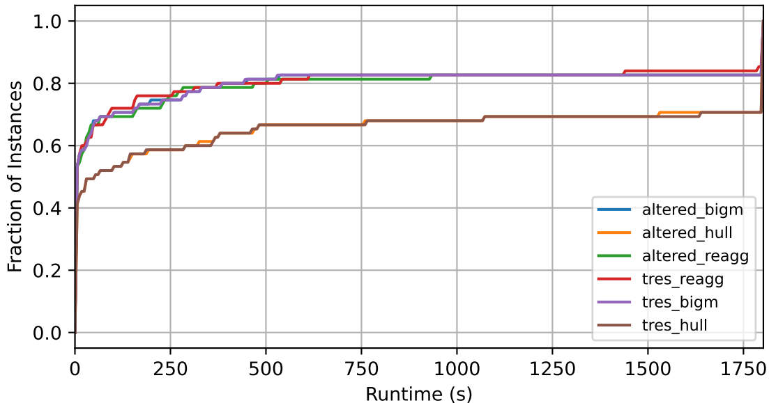
Performance Profile (Runtime Only)
