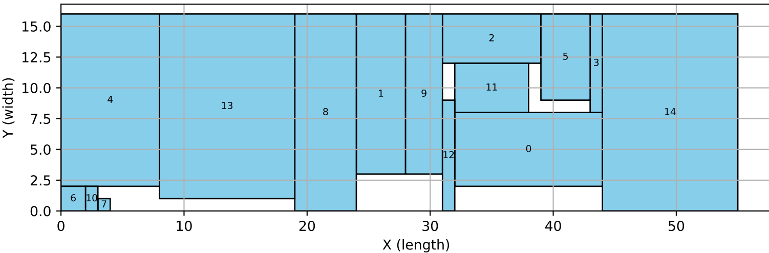
15_1 | tres | bigm
