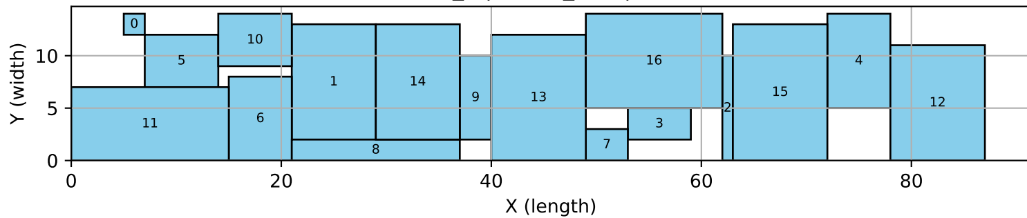
17_4 | reagg_tres | MIP
