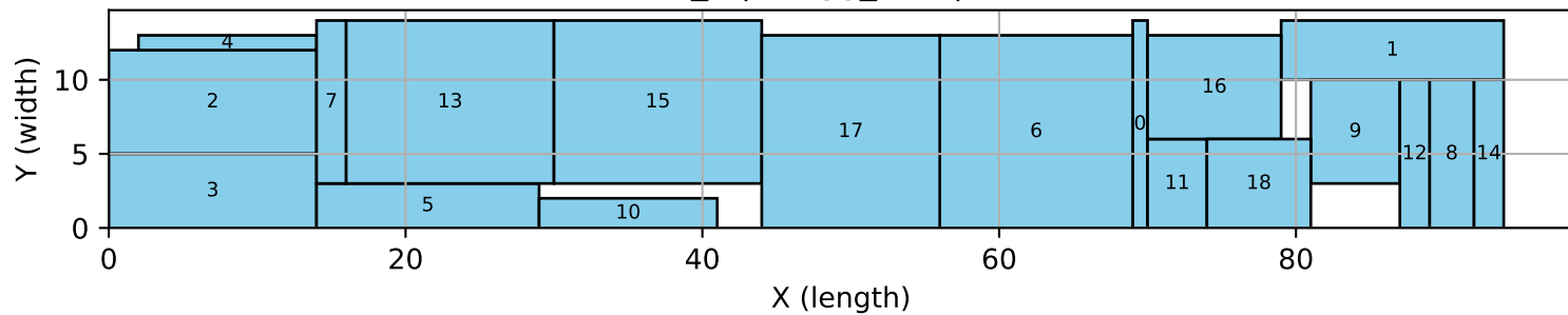
19_2 | reagg_tres | MIP
