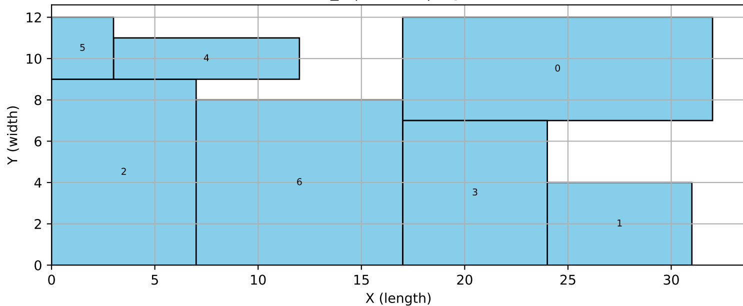
7_1 | altered | bigm
