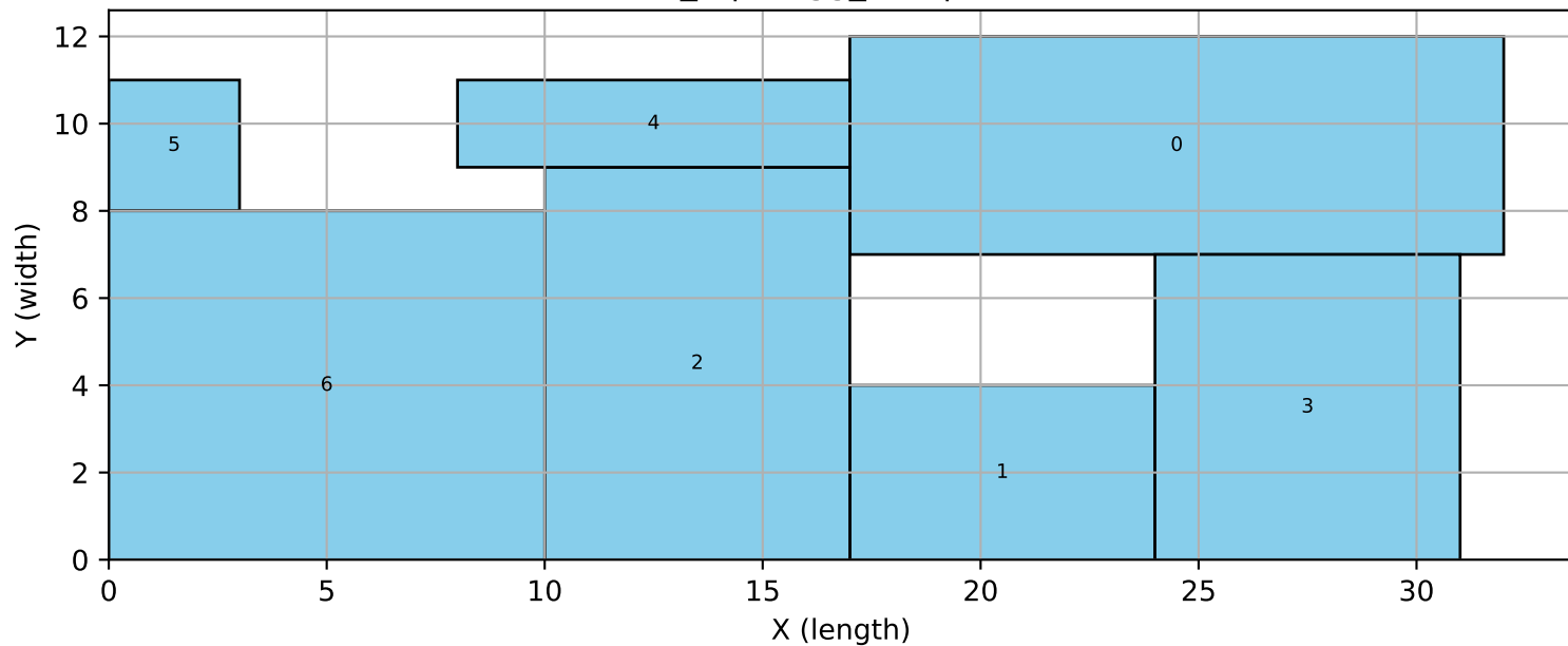
7_1 | reagg_tres | MIP
