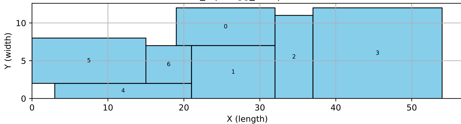
7_3 | reagg_tres | MIP
