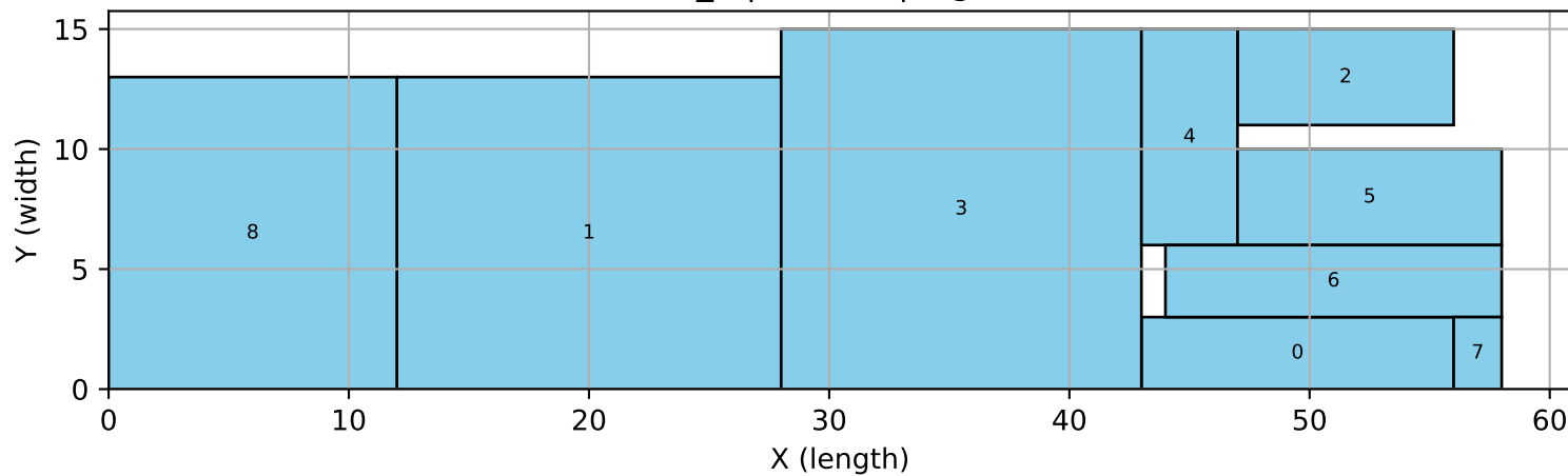
9_5 | altered | bigm
