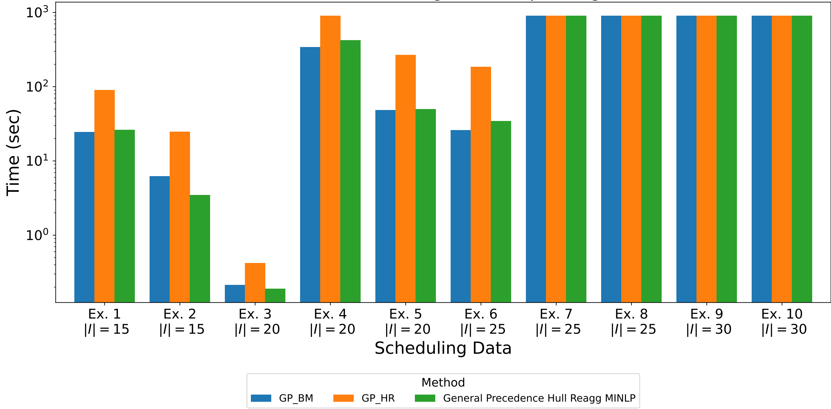
Benchmark Results for Single Unit Sequencing Problem
