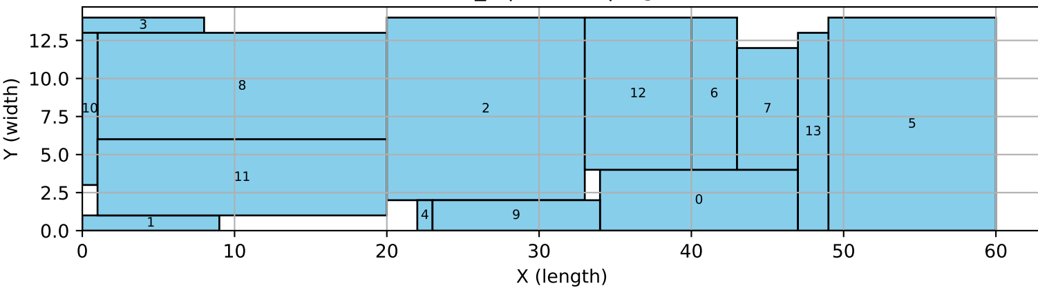
14_7 | altered | bigm
