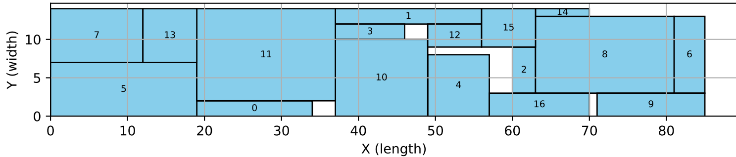
17_7 | reagg | MIP
