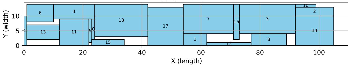
19_6 | reagg | MIP
