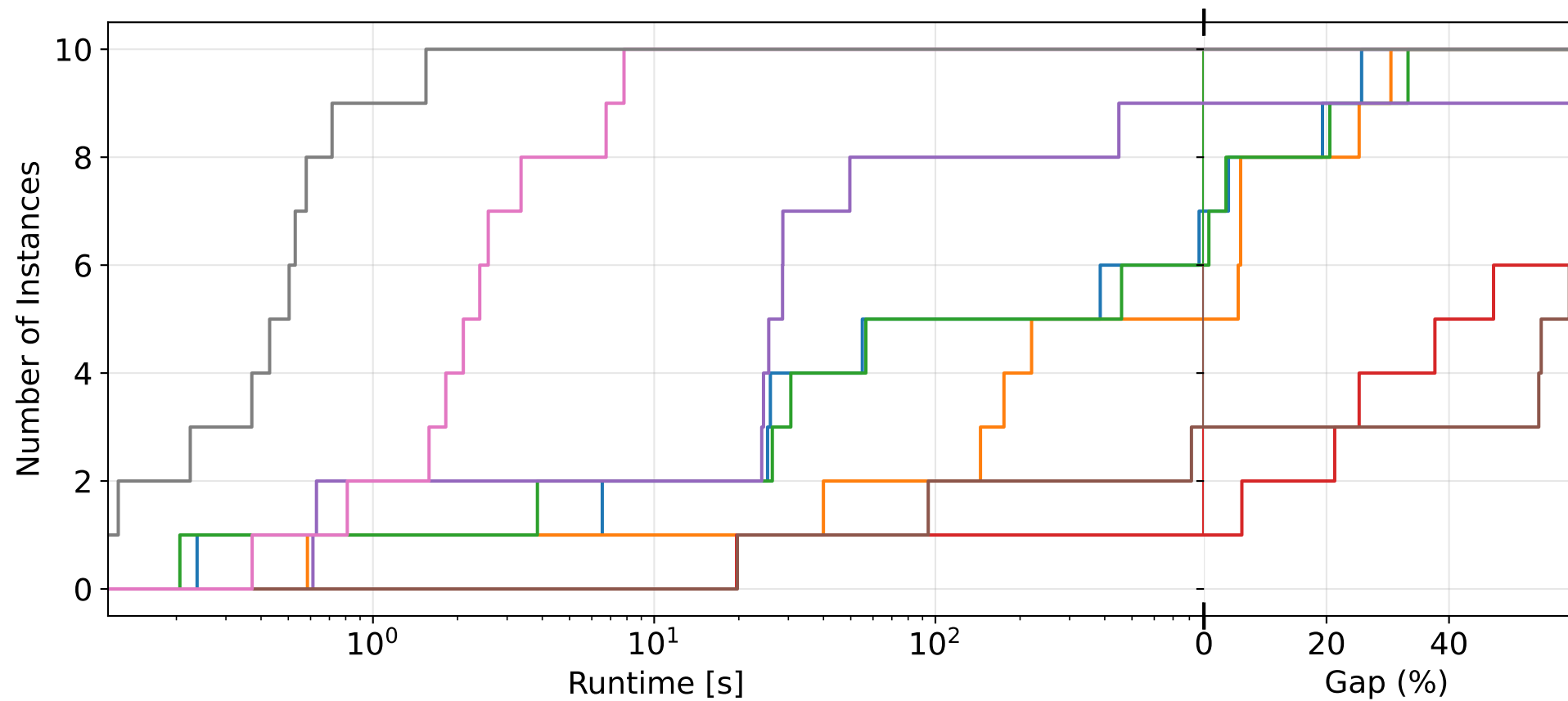
Absolute Performance Profile of Single-Unit Scheduling Reformulations
