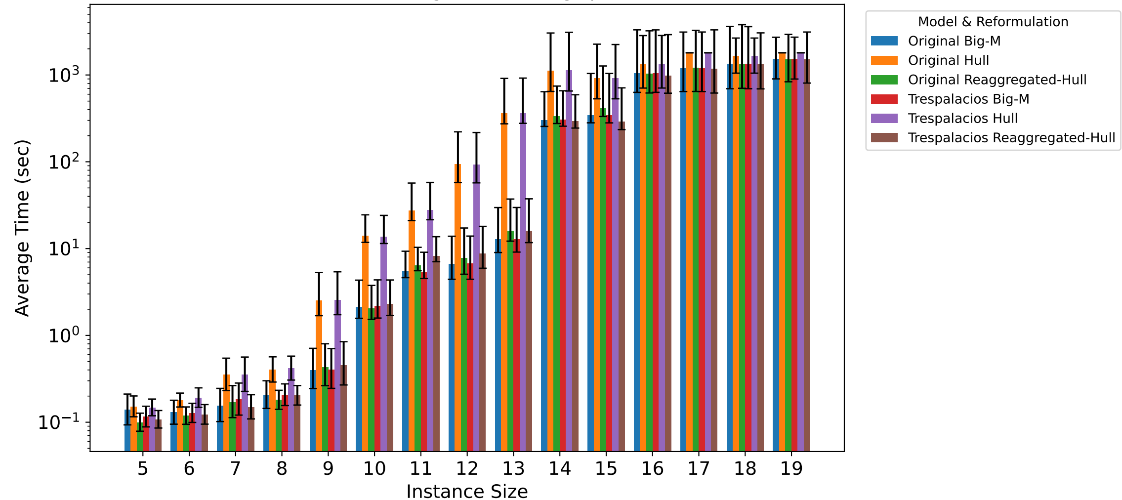
Average Solve Time by Size & Reformulation (5 Cases Averaged, \pm 1\sigma in log-space)
