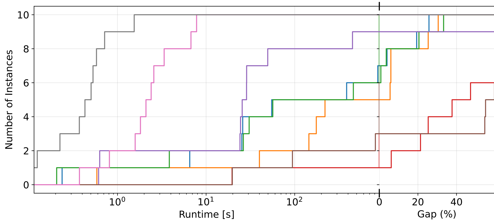
Absolute Performance Profile of Single-Unit Scheduling Reformulations using Gurobi
