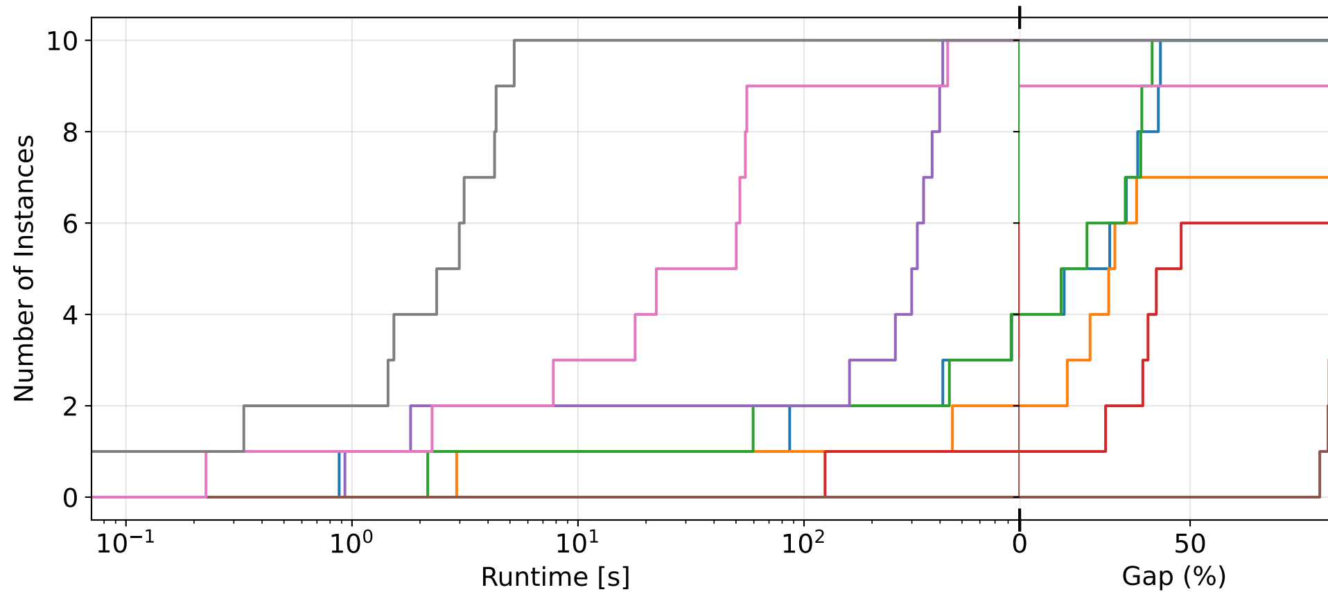
Absolute Performance Profile of Single-Unit Scheduling Reformulations using HiGHS
