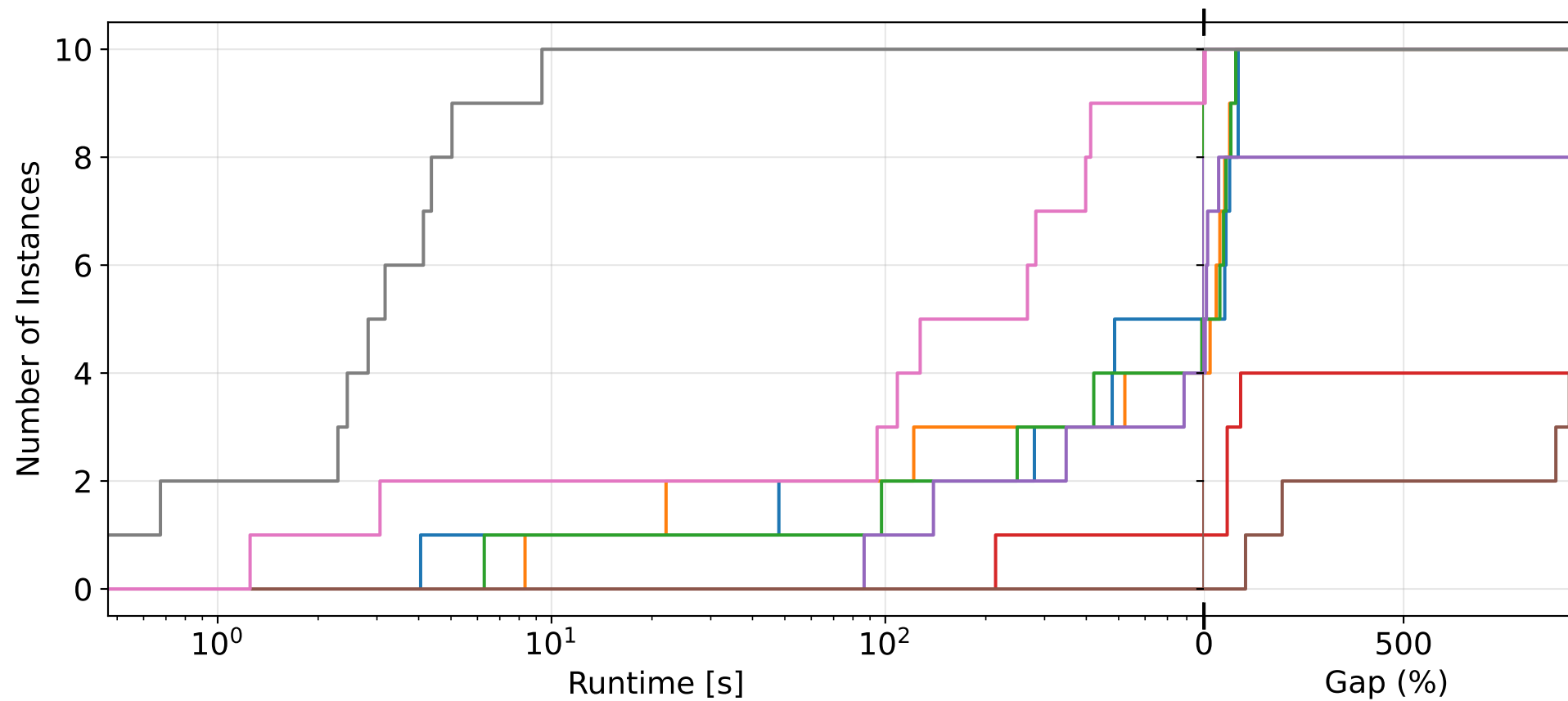
Absolute Performance Profile of Single-Unit Scheduling Reformulations using SCIP
