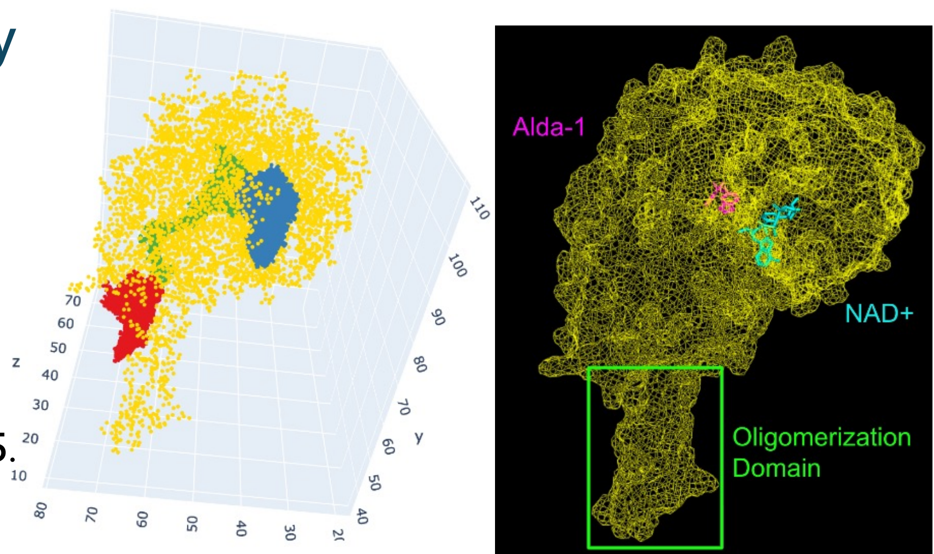
Figure 5: Docking Position of >0.8 Similarity Compounds (Red, blue, and green; yellow for ALDH2)
