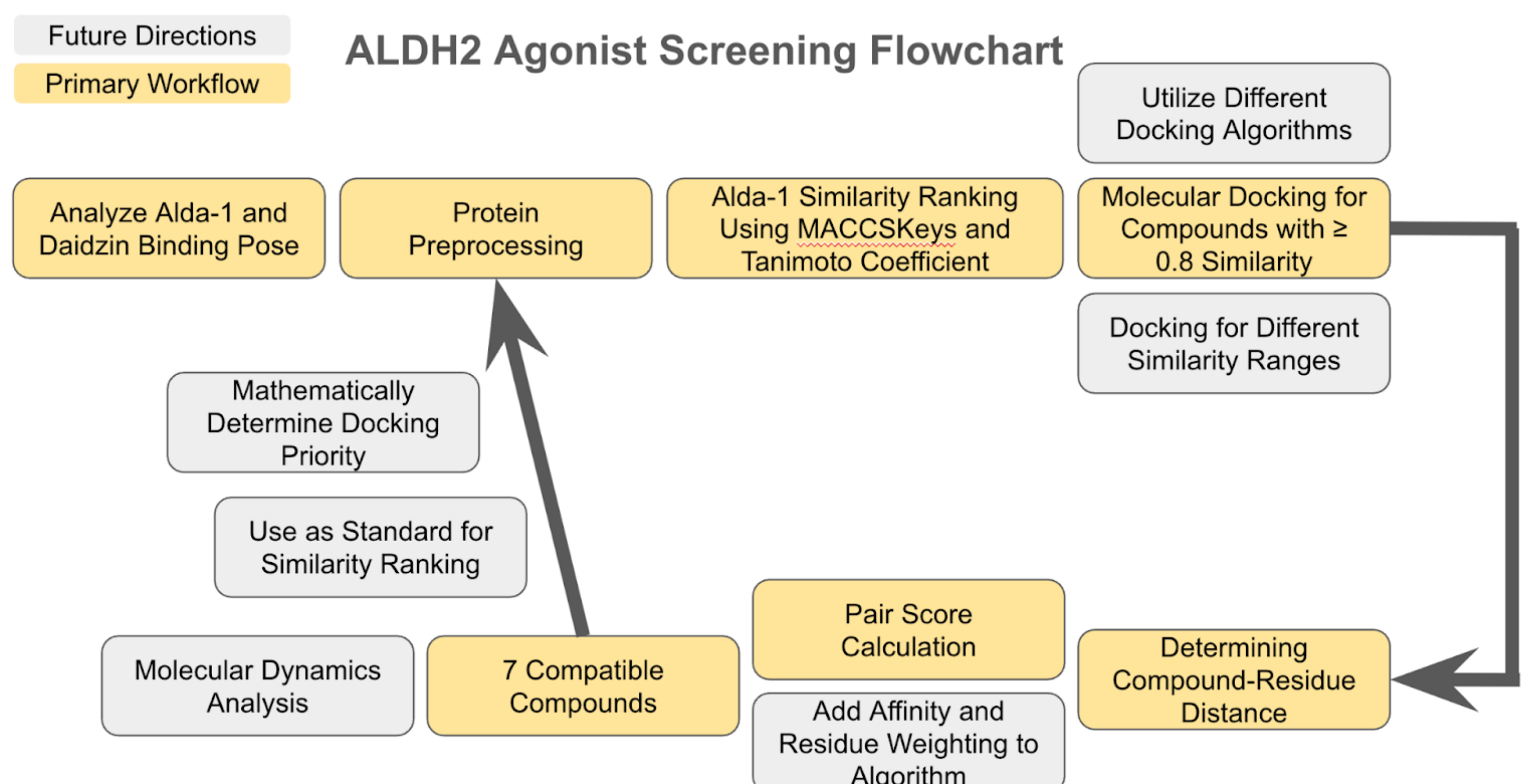
Figure 2: ALDH2 Agonist Screening Flowchart
