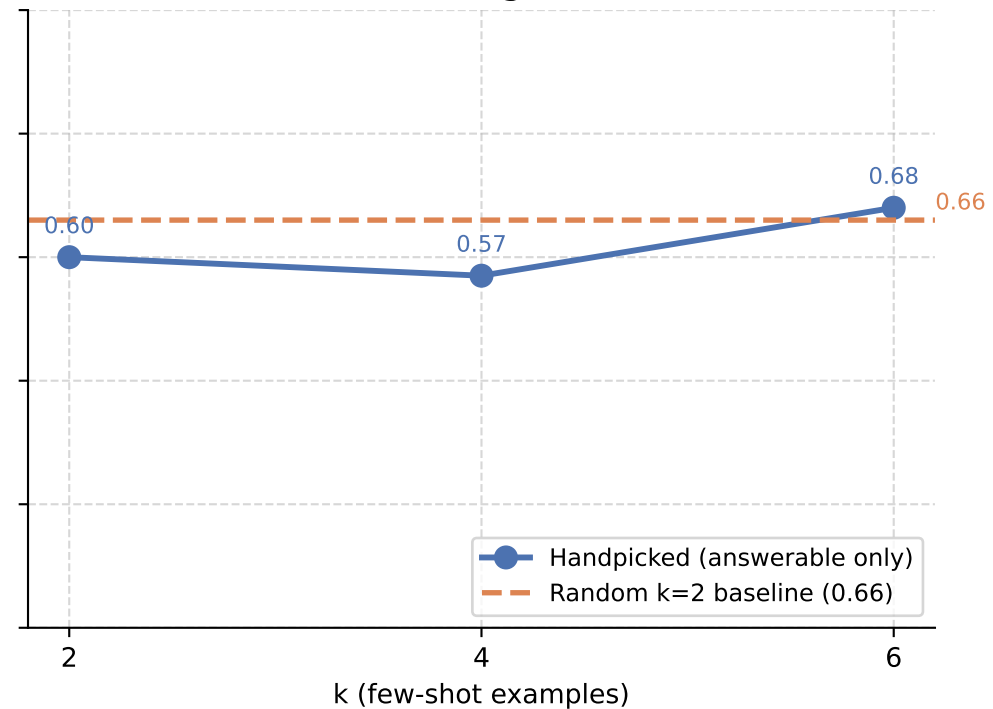
BoundingDocs
