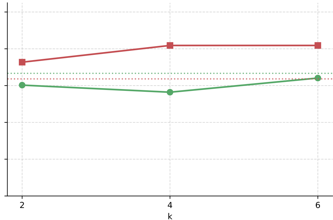
BoundingDocs
