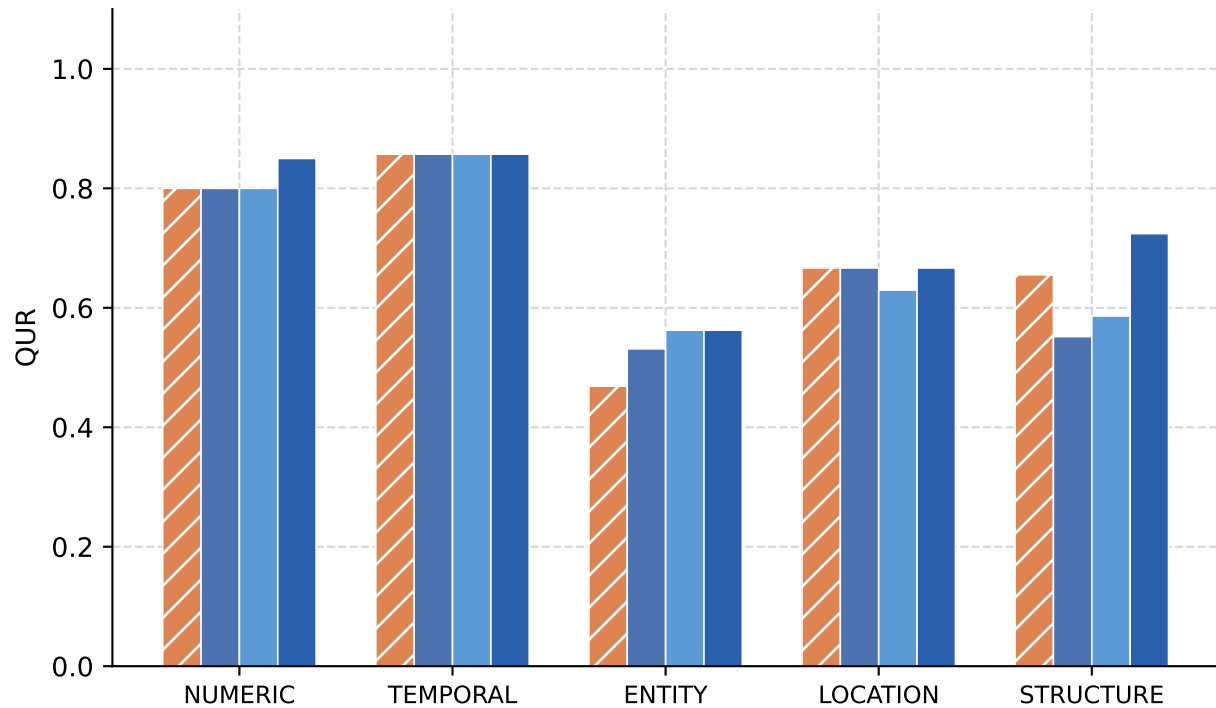
BoundingDocs
