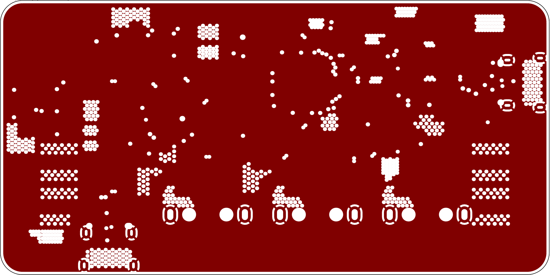
Int4 (GND) (Scale 5:2)
