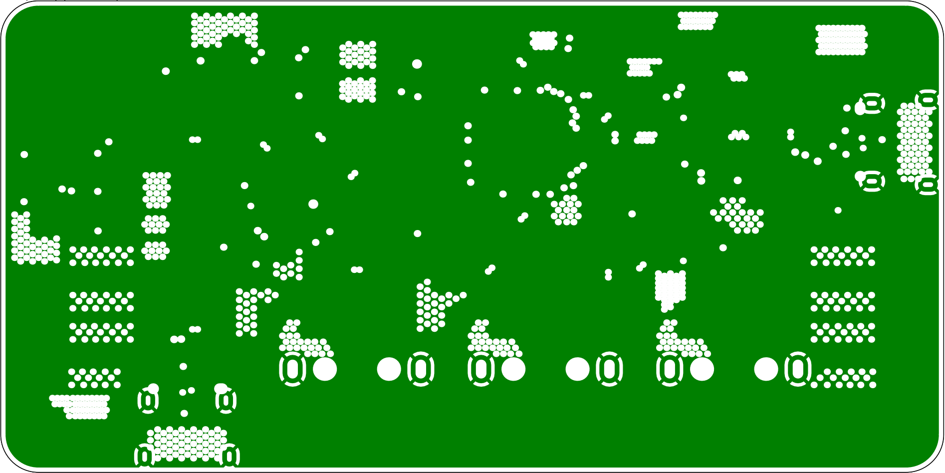
Int1 (GND) (Scale 5:2)
