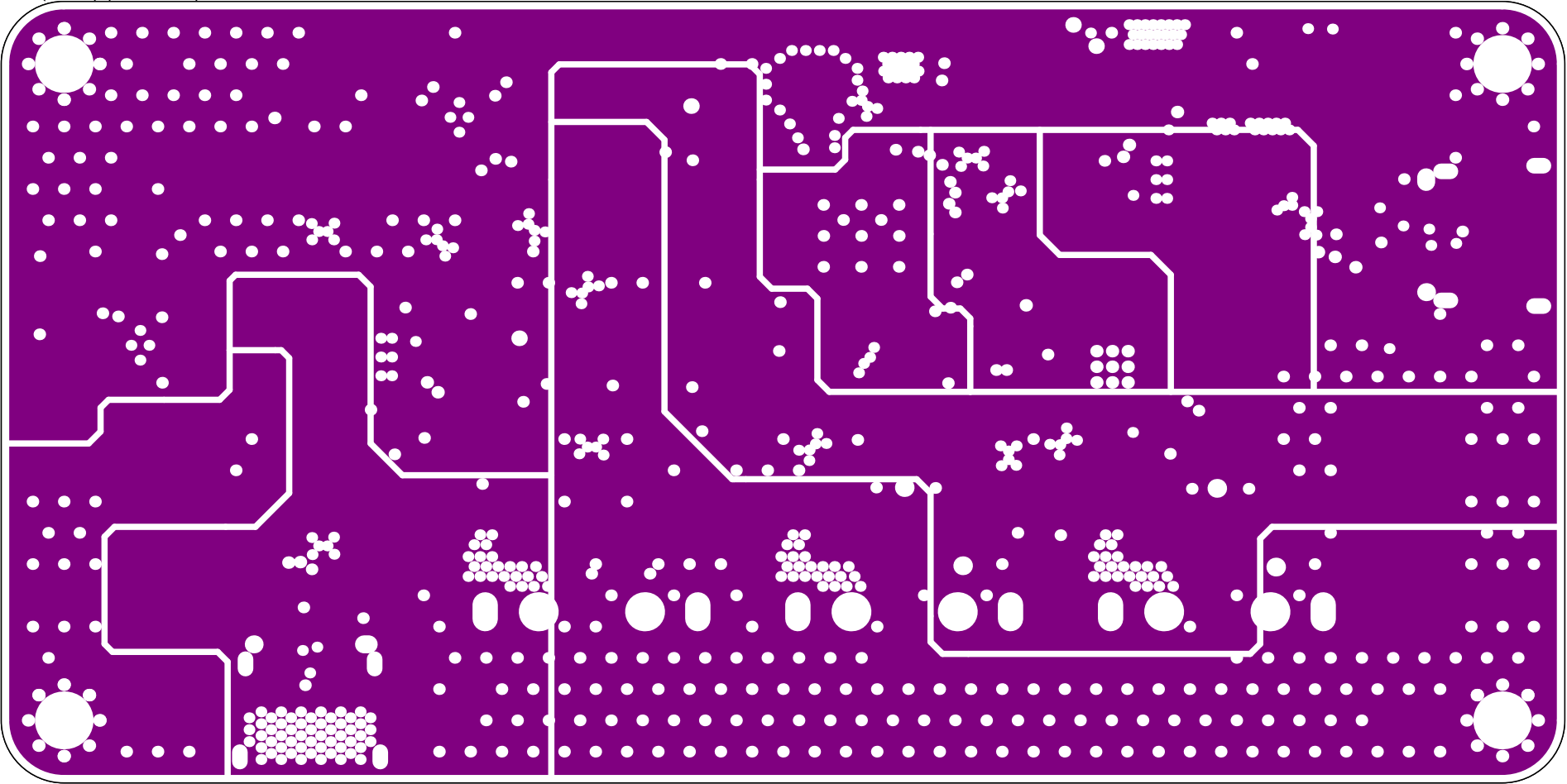
Int3 (PWR) (Scale 5:2)
