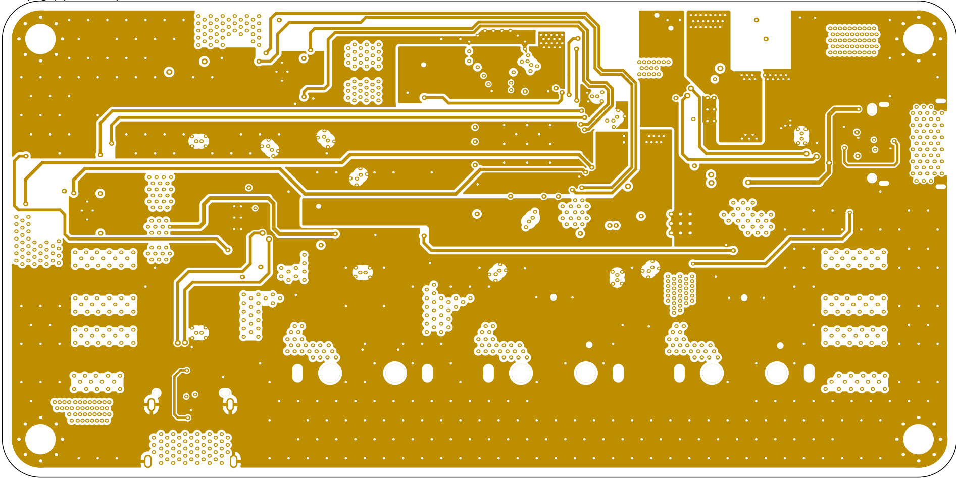
Int2 (Sign) (Scale 5:2)
