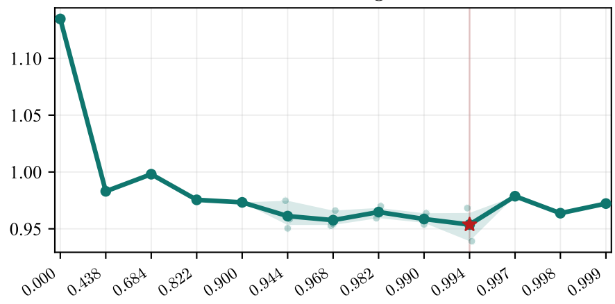
ViT-B/16 on TinyImageNet
