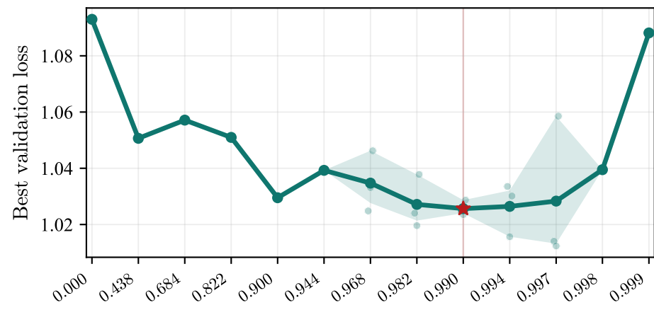
ViT-B/16 on CIFAR-100
