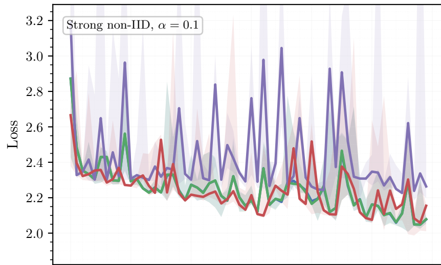
Test loss
