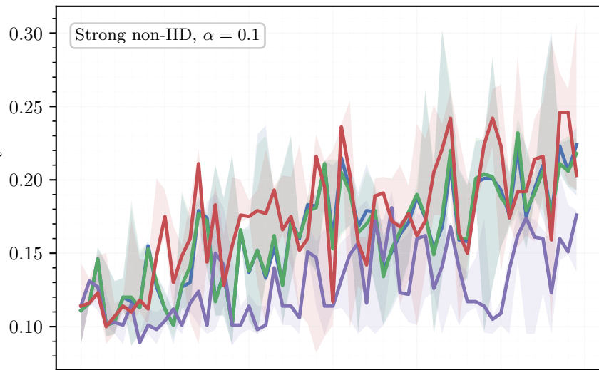
Test accuracy
