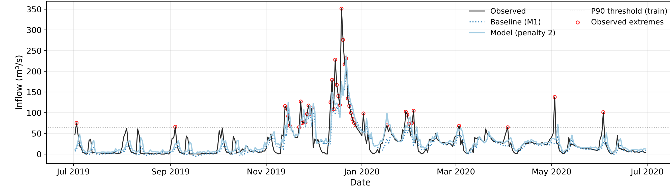
Inflow Forecast 2019 - M2 - Loss: Pinball p=2 - Meta-Learner: None
