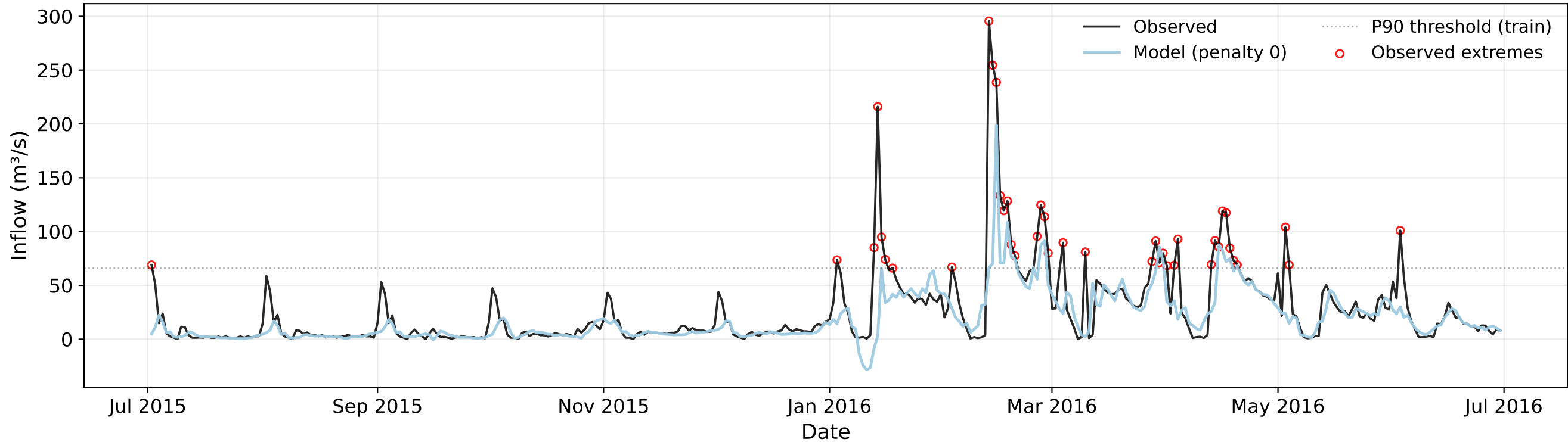
Inflow Forecast 2015 - M1 - Loss: MAE - Meta-Learner: None
