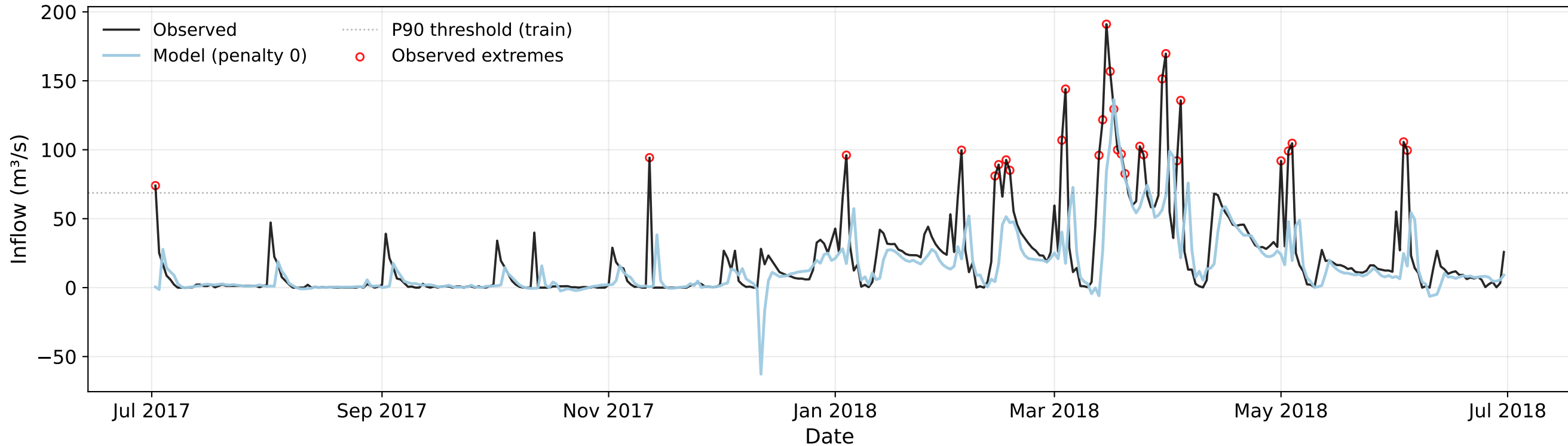
Inflow Forecast 2017 - M1 - Loss: MAE - Meta-Learner: None
