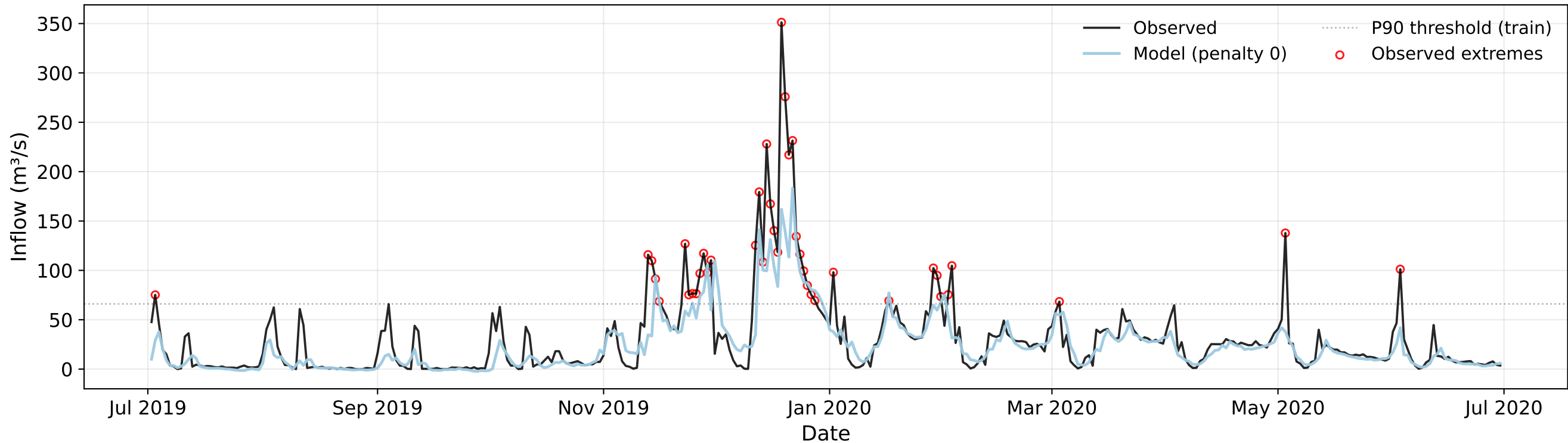
Inflow Forecast 2019 - M1 - Loss: MAE - Meta-Learner: None
