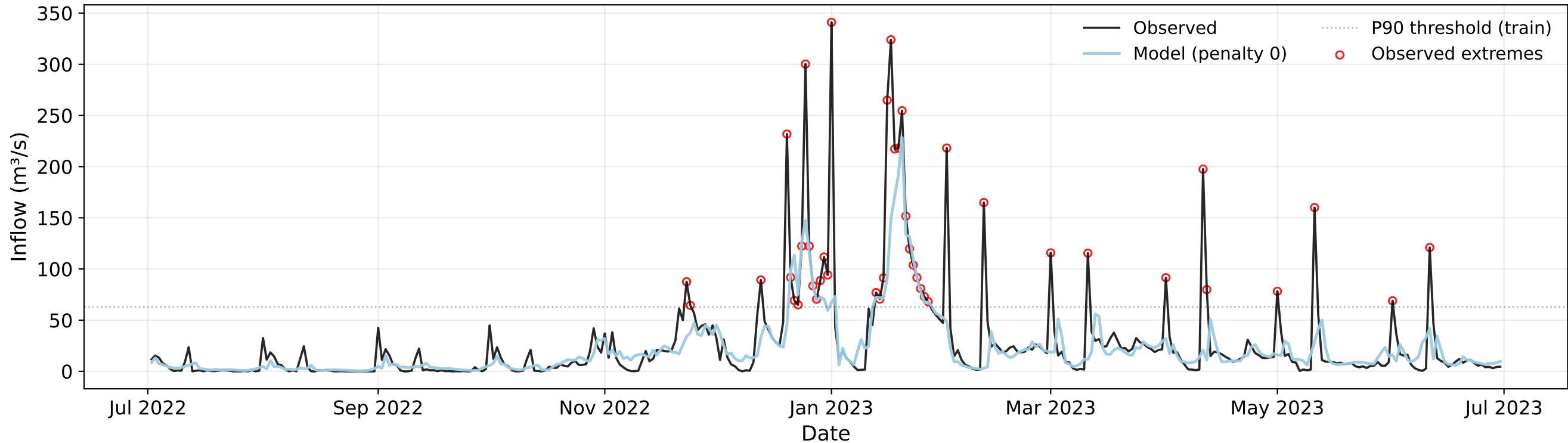
Inflow Forecast 2022 - M1 - Loss: MAE - Meta-Learner: None
