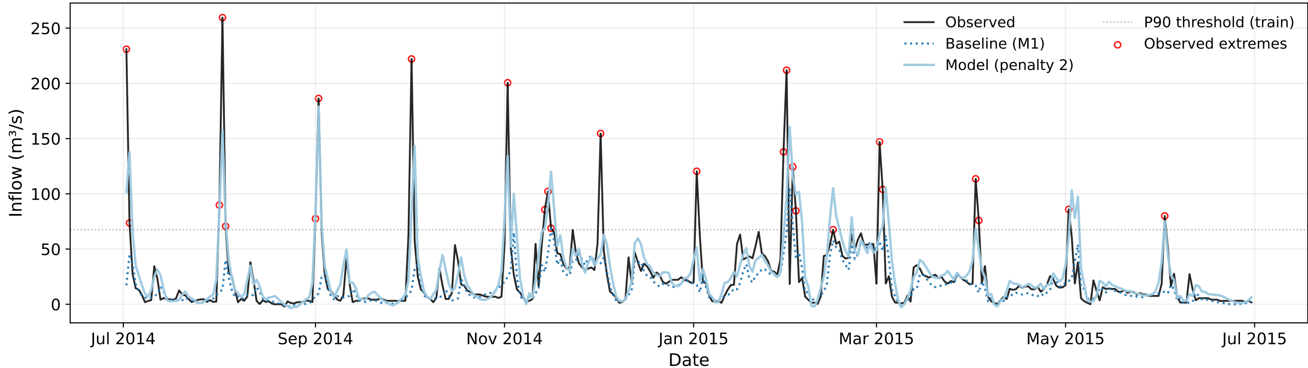
Inflow Forecast 2014 - M2 - Loss: Pinball p=2 - Meta-Learner: None
