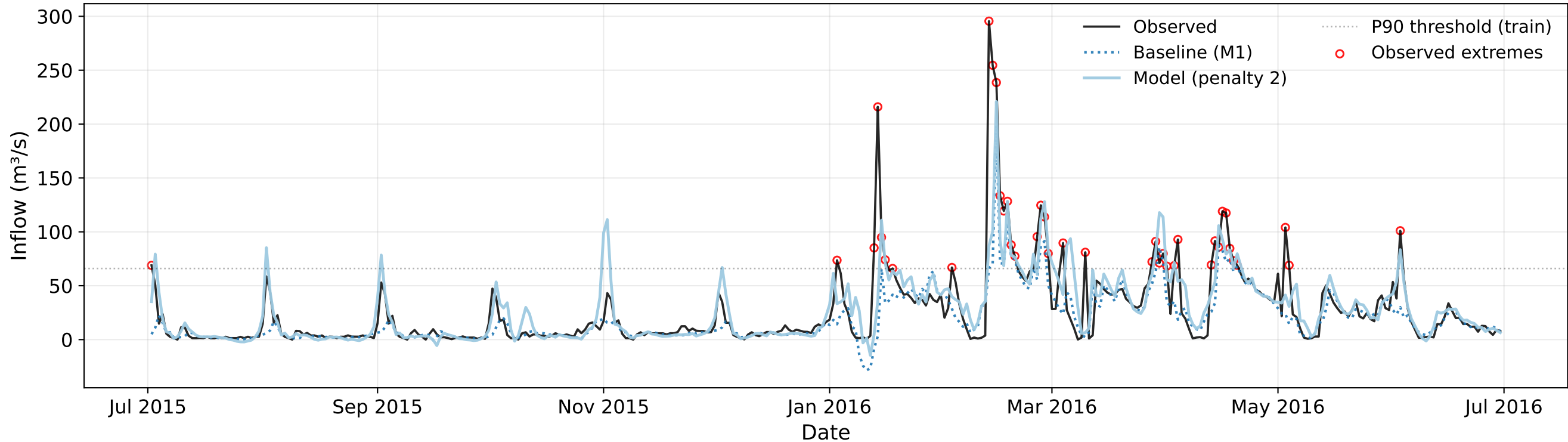
Inflow Forecast 2015 - M2 - Loss: Pinball p=2 - Meta-Learner: None
