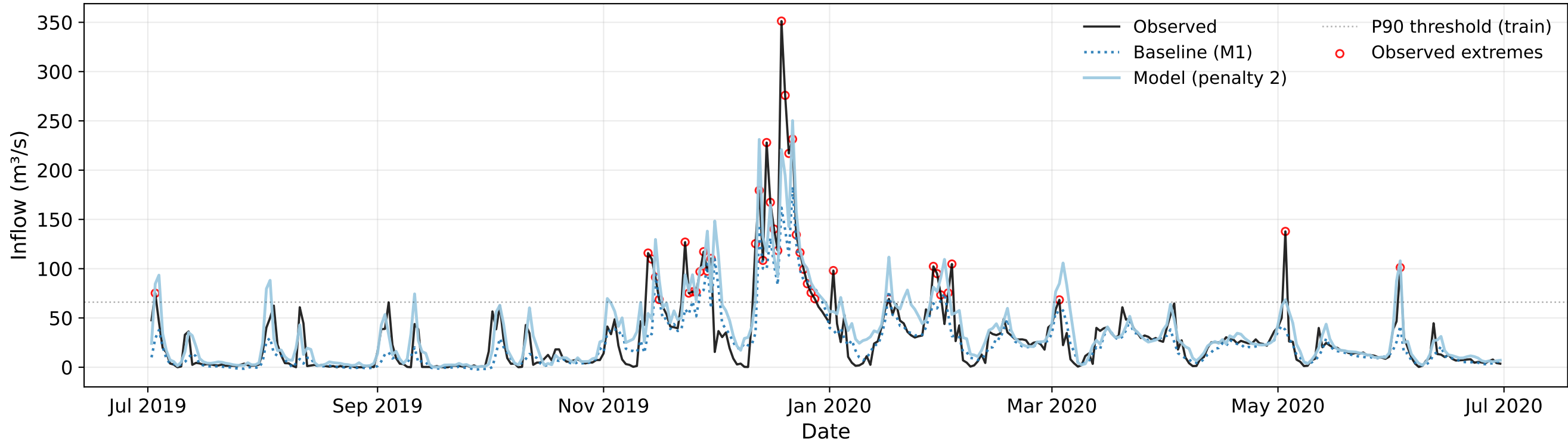
Inflow Forecast 2019 - M2 - Loss: Pinball p=2 - Meta-Learner: None
