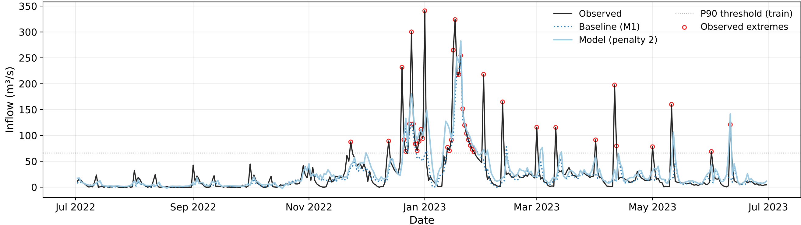
Inflow Forecast 2022 - M2 - Loss: Pinball p=2 - Meta-Learner: None
