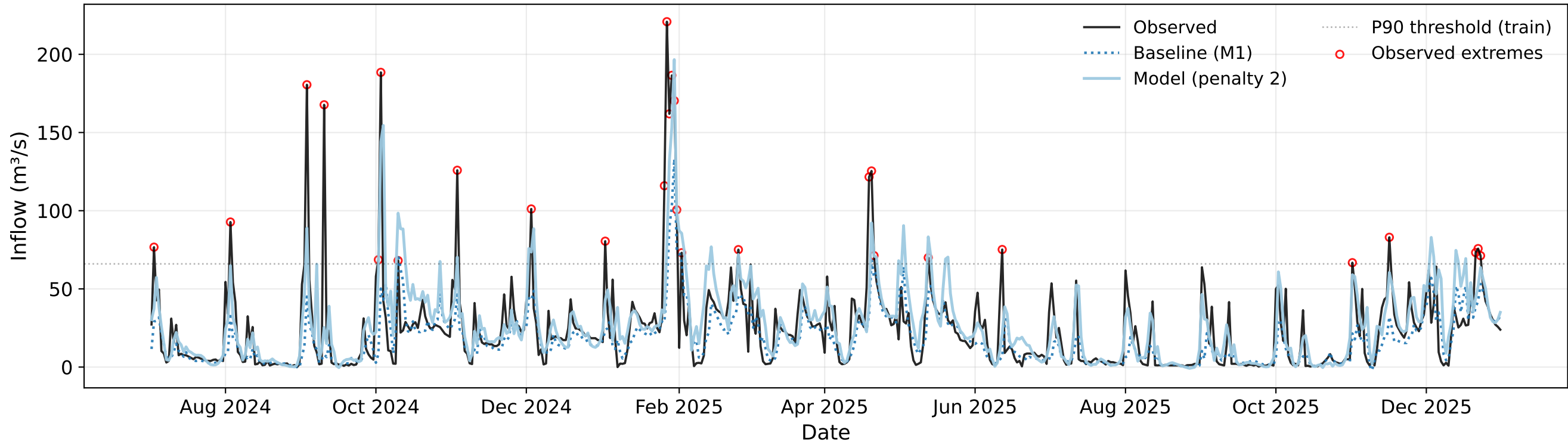
Inflow Forecast 2025 - M2 - Loss: Pinball p=2 - Meta-Learner: None
