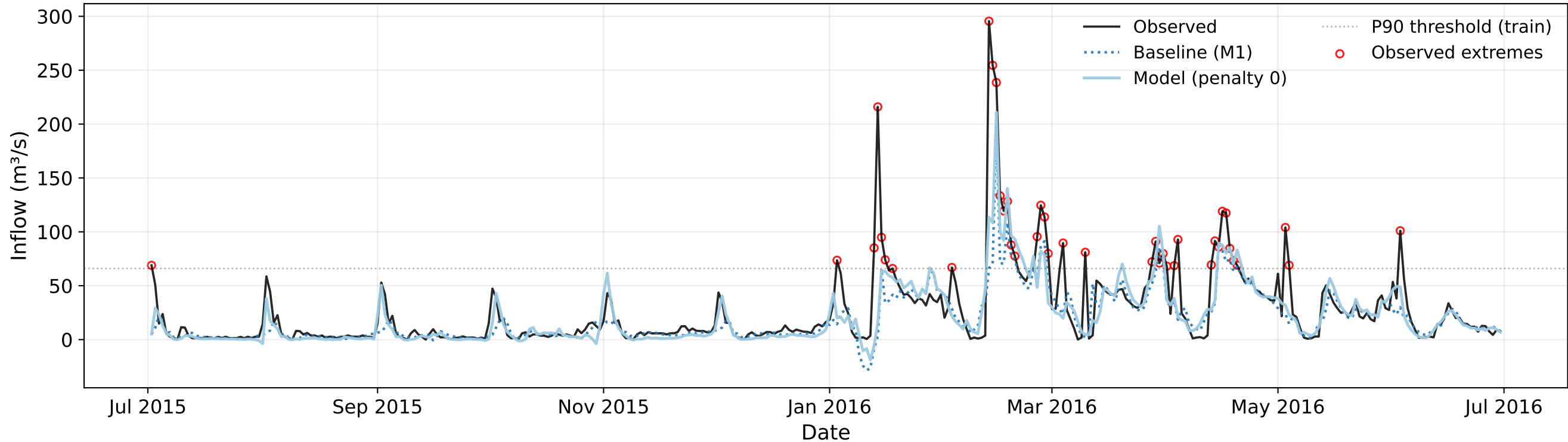
Inflow Forecast 2015 - M3 - Loss: MAE - Meta-Learner: None
