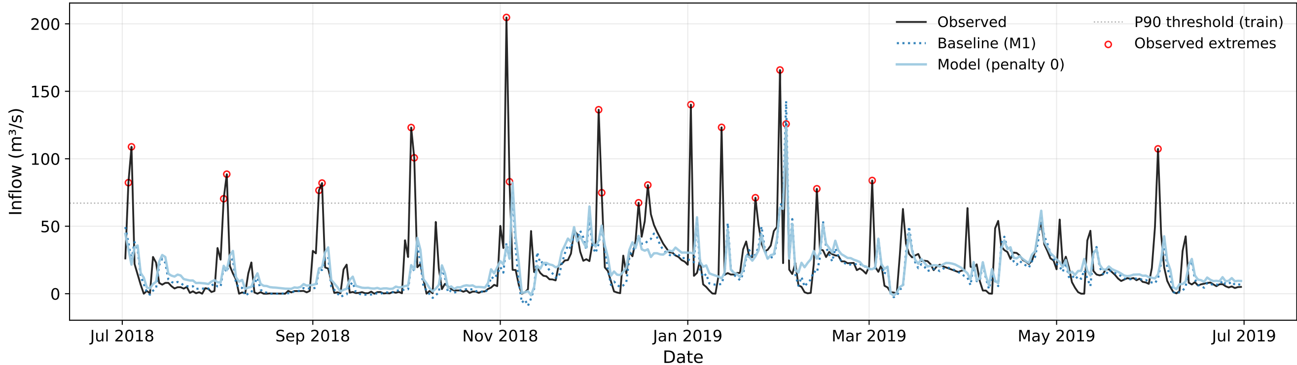
Inflow Forecast 2018 - M3 - Loss: MAE - Meta-Learner: None
