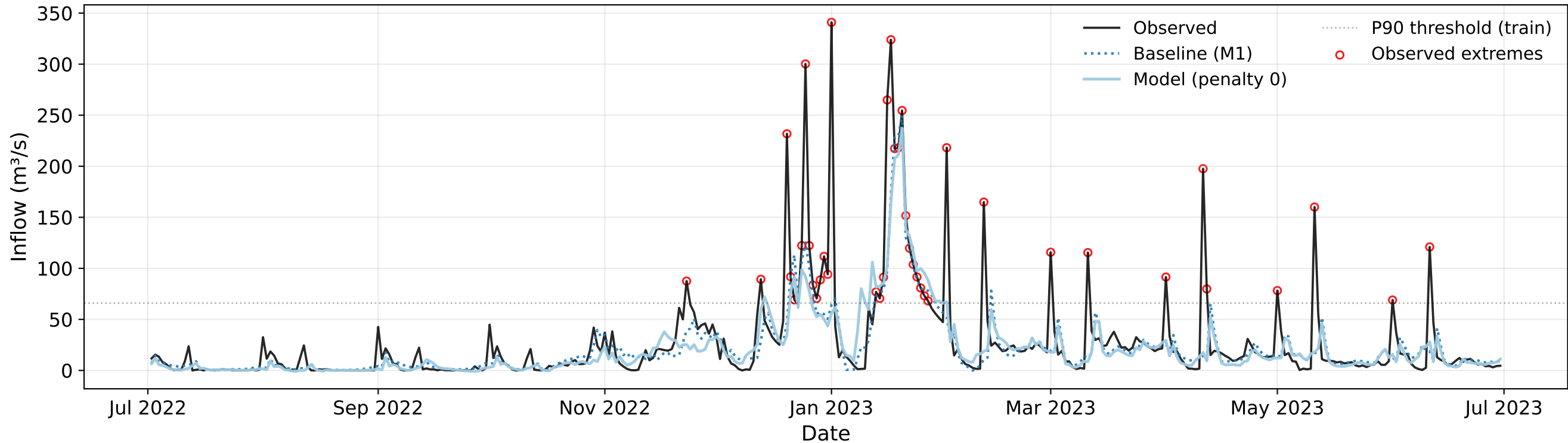
Inflow Forecast 2022 - M3 - Loss: MAE - Meta-Learner: None
