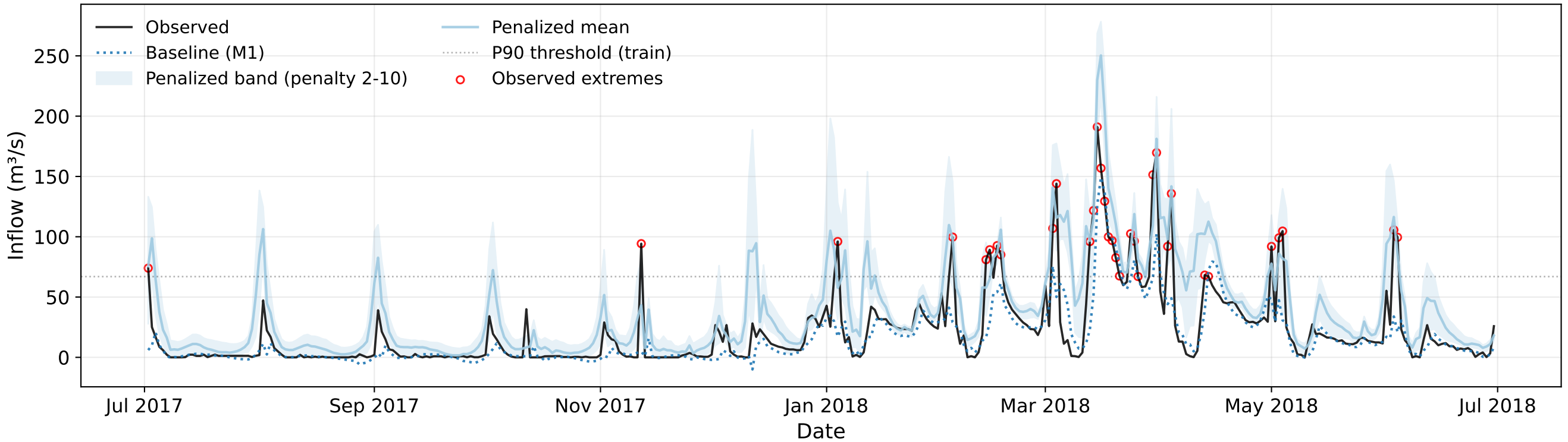
Inflow Forecast 2017 - M4 - Loss: Pinball p=2-10 - Meta-Learner: None
