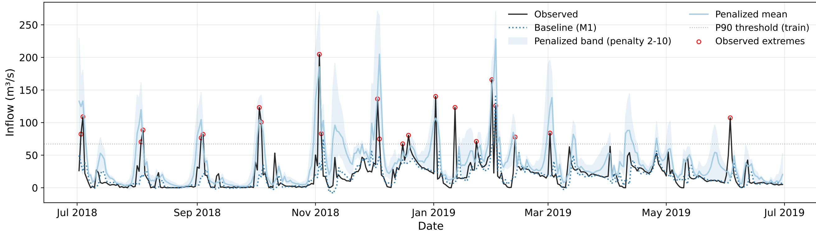
Inflow Forecast 2018 - M4 - Loss: Pinball p=2-10 - Meta-Learner: None
