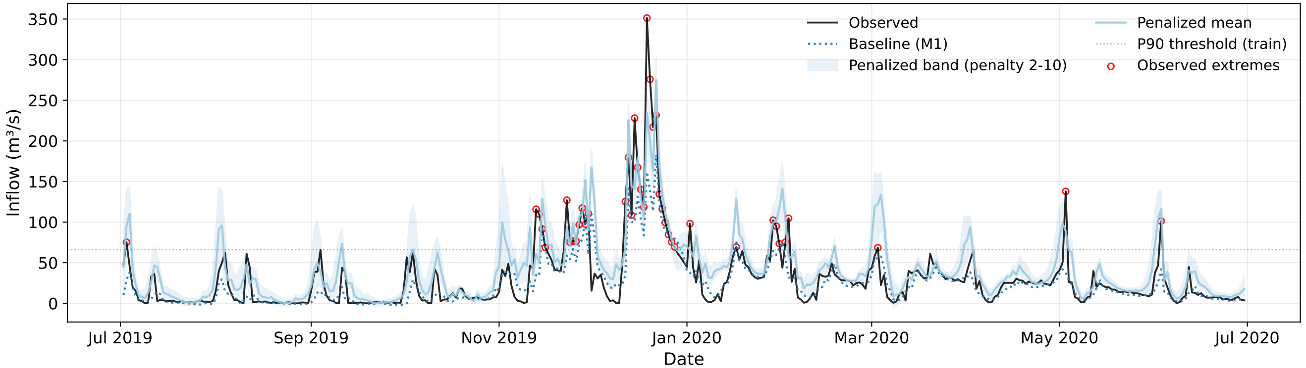
Inflow Forecast 2019 - M4 - Loss: Pinball p=2-10 - Meta-Learner: None
