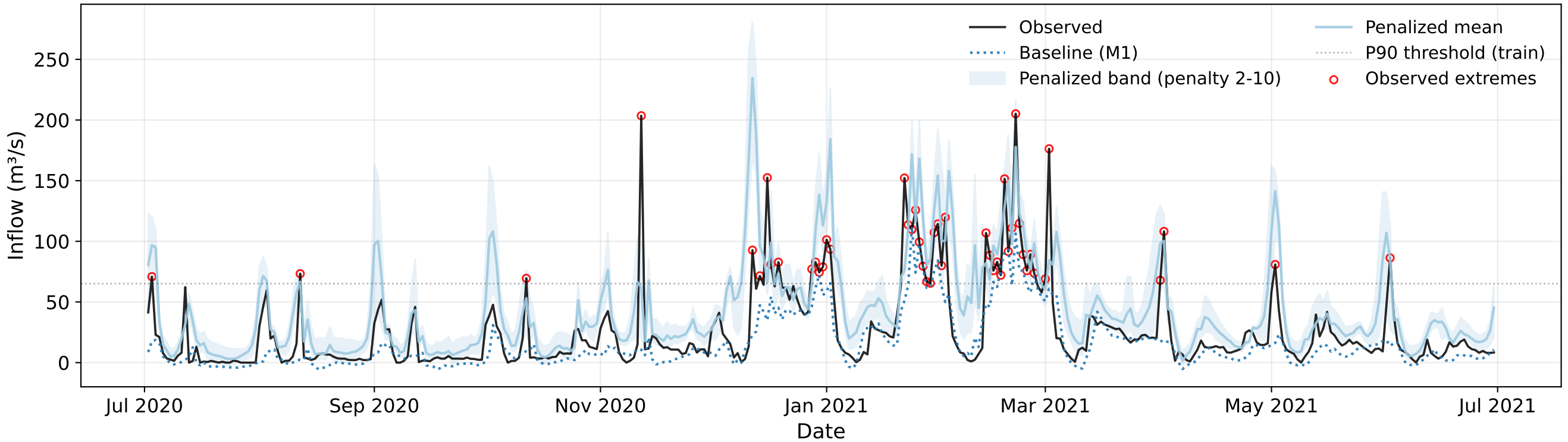
Inflow Forecast 2020 - M4 - Loss: Pinball p=2-10 - Meta-Learner: None
