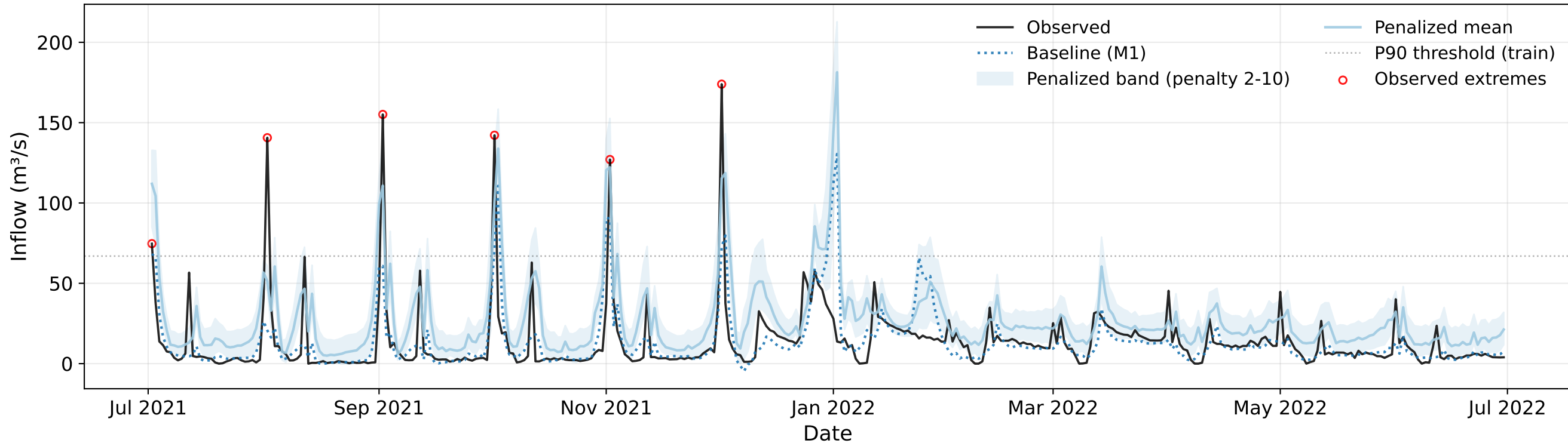
Inflow Forecast 2021 - M4 - Loss: Pinball p=2-10 - Meta-Learner: None
