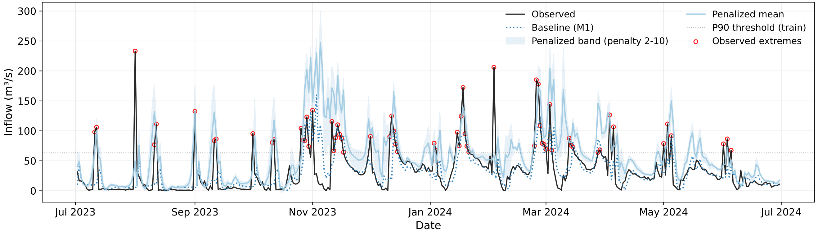
Inflow Forecast 2023 - M4 - Loss: Pinball p=2-10 - Meta-Learner: None
